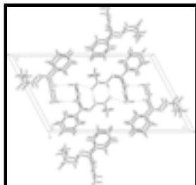
Fig. 2. A packing diagram of the molecule of the title compound, view down b axis. Hydrogen bonds are shown as dashed lines.
